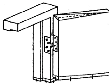
Rising Butt Hinge - special preparation at top of door
