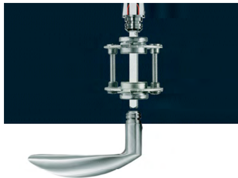
Lever furniture with back-to-back bolts (plan view)
