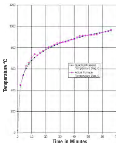
Time/temperature curve BS EN 1634-1
