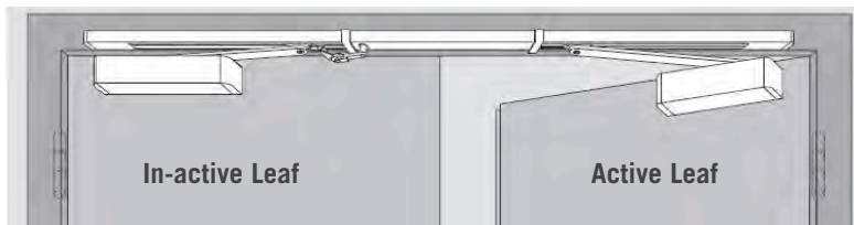
Overhead closer with integral co-ordinator
