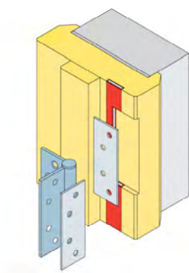
Pads behind hinge blades
