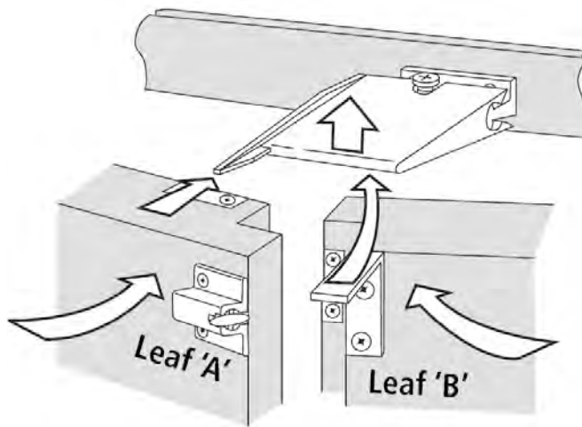
Gravity arm co-ordinator
