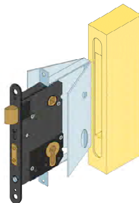
Full gasket for mortise lock
